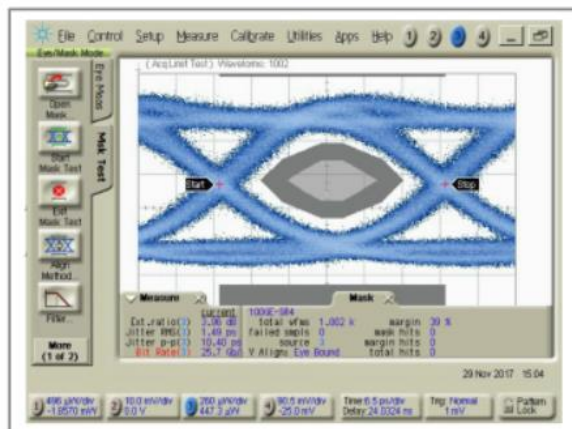
Eye Pattern
